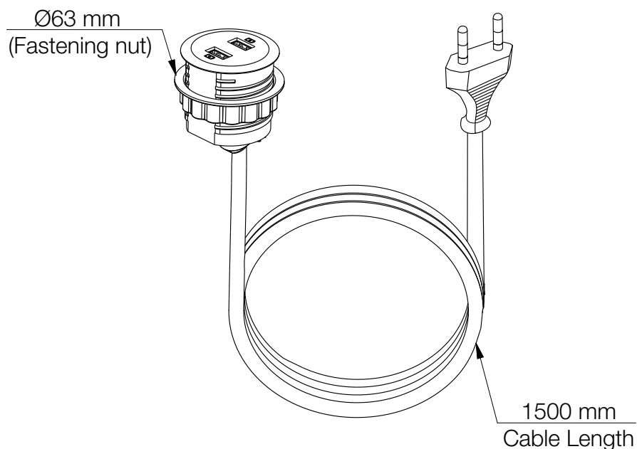
Oriented view (Grommet, nut & cable)
