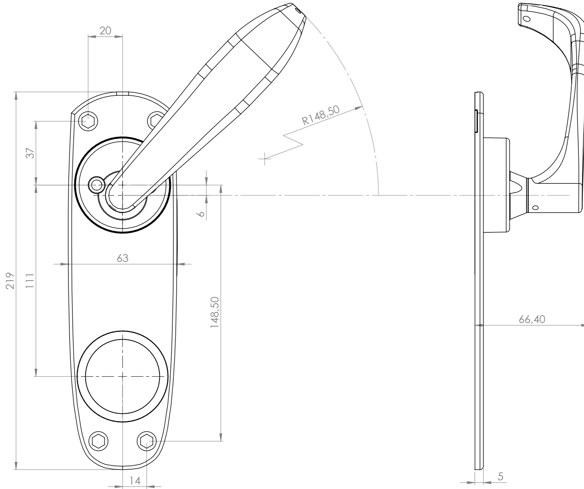
Drawing of 791 model (792 has no hole for door handle)
