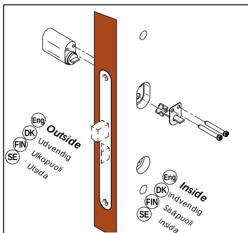
Single cylinder with thumb turn Enkelt cylinder med vrider
