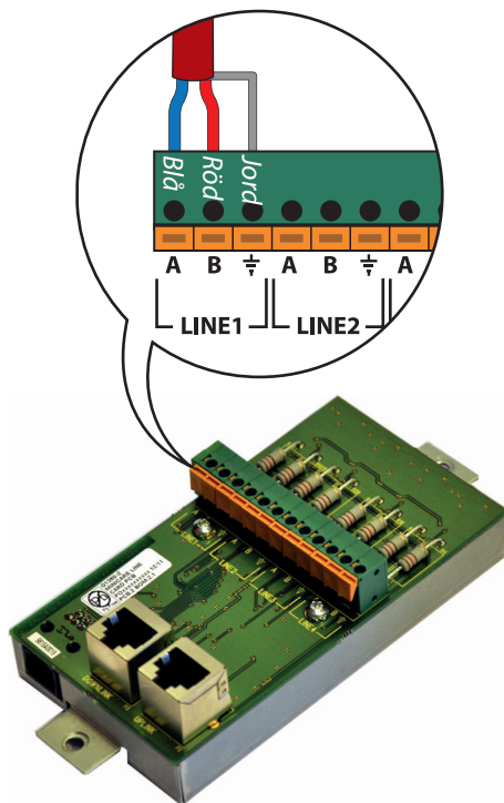
Expansionskort SAC-SAFE-TEL C2CEK4
