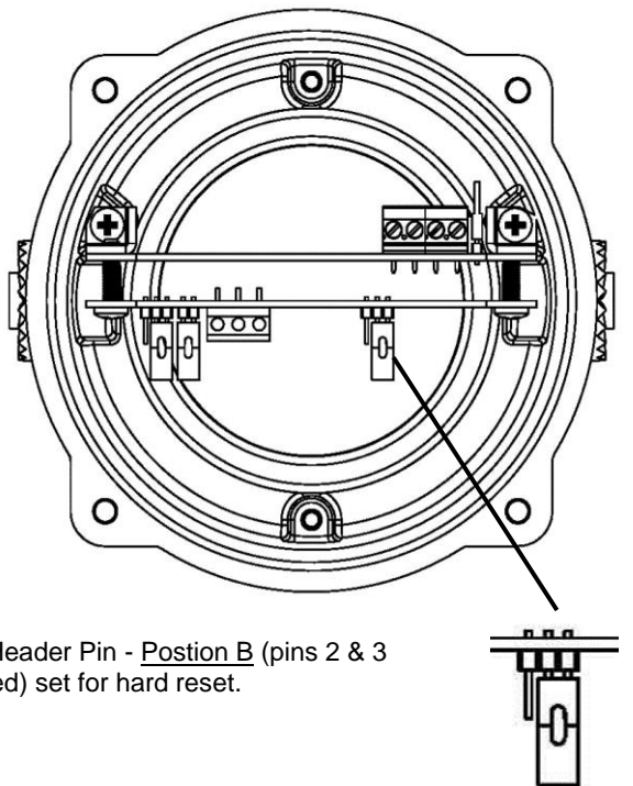
Fig 10 – Jumper Settings
