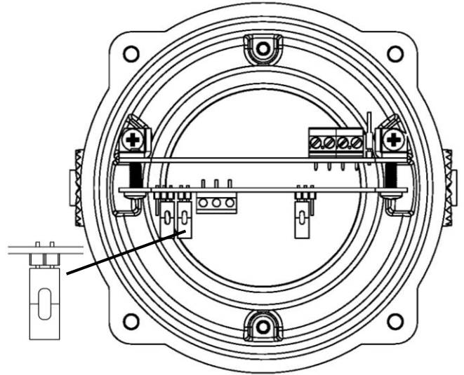
J1 Header Pin - Position B (pins 1 & 2 linked) removes TB1 Current sense resistor out of circuit.
