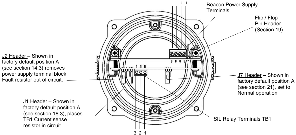
Figure 5 – Terminals and header pins for beacon
