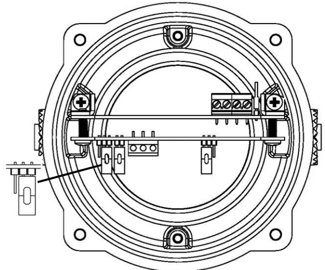
J2 Header Pin - Position B (pins 2 & 3 linked) places power supply TB Fault resistor & RLY 1-2 in
