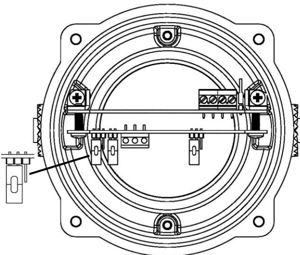
J2 Header Pin - Position A , Factory default position (pins 1 & 2 linked) removes power supply TB Fault resistor & RLY 1-2 out of circuit.
