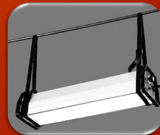
Strap L=800mm, B=19mm Art. No. 106865 or Strap with a loop L=100mm, B=25mm Art. No. 107865
