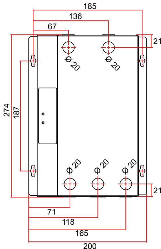
Knockouts: back
