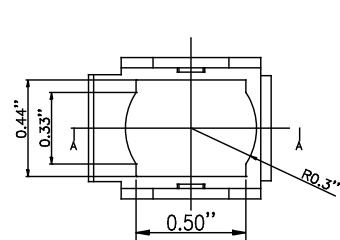
MODULE DRAWING(UNIT:INCH)
