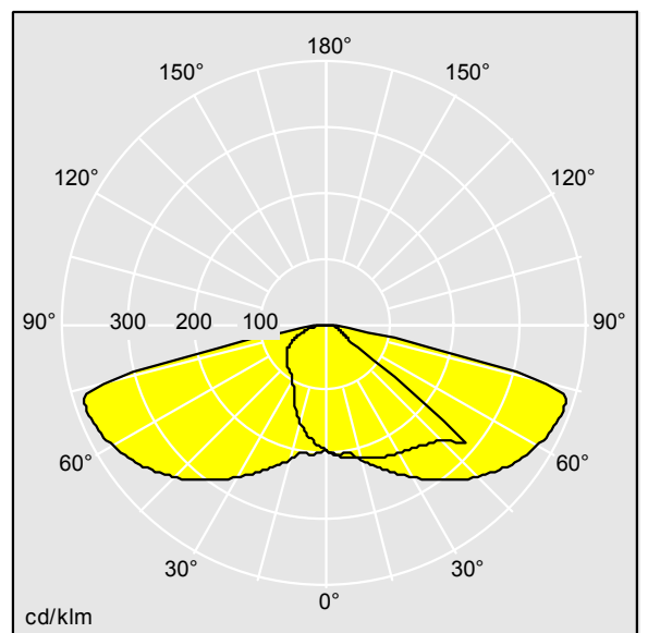
TLLA_IP12L105NR740G34_DC.ltd
