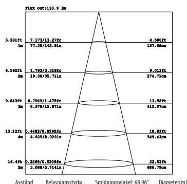
Illuminance-Distance Curve
