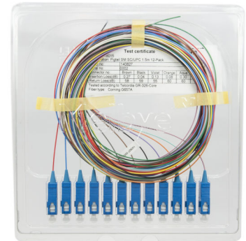
Pigtail SM SC/UPC 1.5m 12-pack
